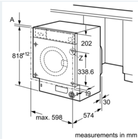
Dimensioned drawings
