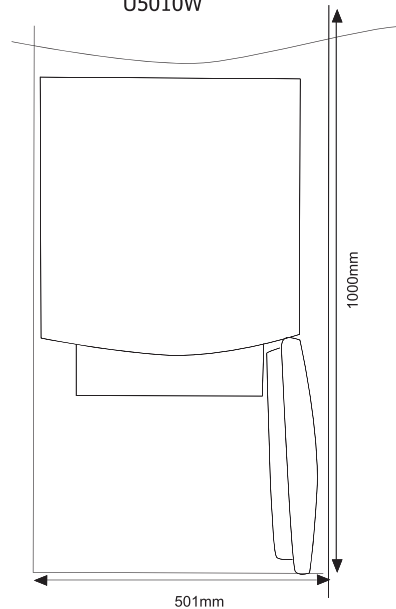
Total space required in use U5010W
