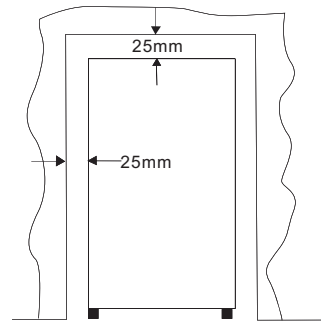
Total space required in use U5010W
